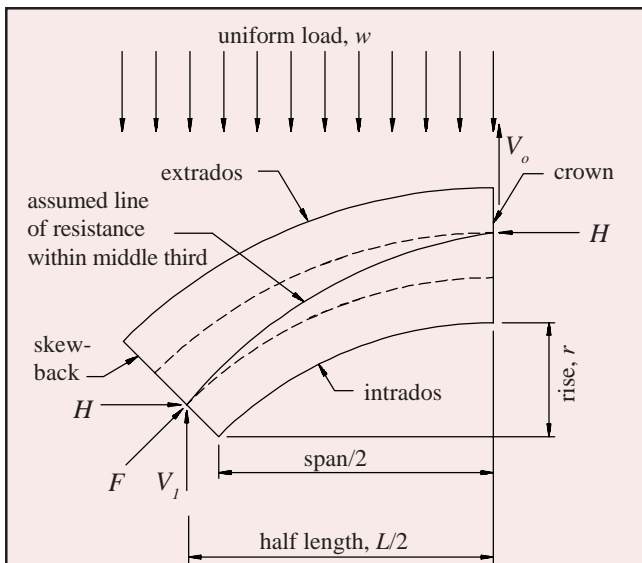
Figure 2—Assumed Conditions for Static Analysis of Small Concrete Masonry Arch
