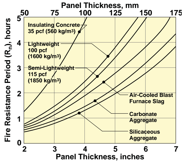
Figure 2 Fire Resistance Periods for Other Concrete Panels
