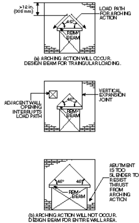
Conditions for Arching Action FIG. 3
